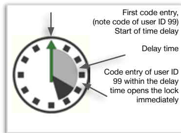
Opening with bypassing of activated time delay
